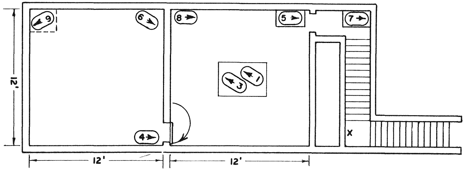
Fig. 6.1--Floor plan of the shelter, showing placement of the pigs. The arrow indicates the head of the animal. The stairway was oriented toward GZ. Direct thermal radiation occurred at X on the landing since the top of the tower was on a line of sight from this position.
